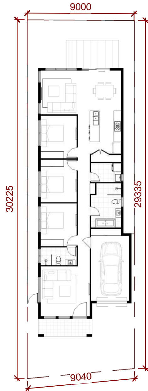
LOT PLAN
