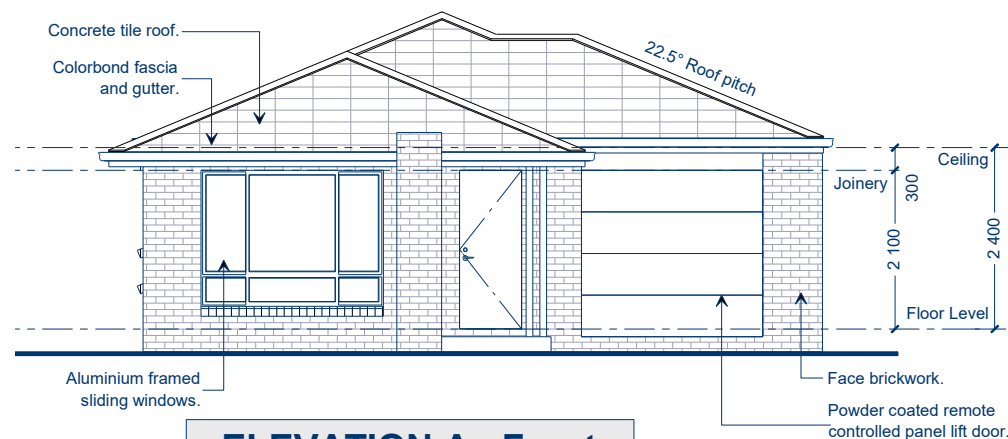
ELEVATION A - Front
