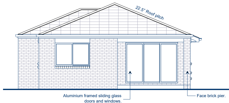
ELEVATION C - Rear
