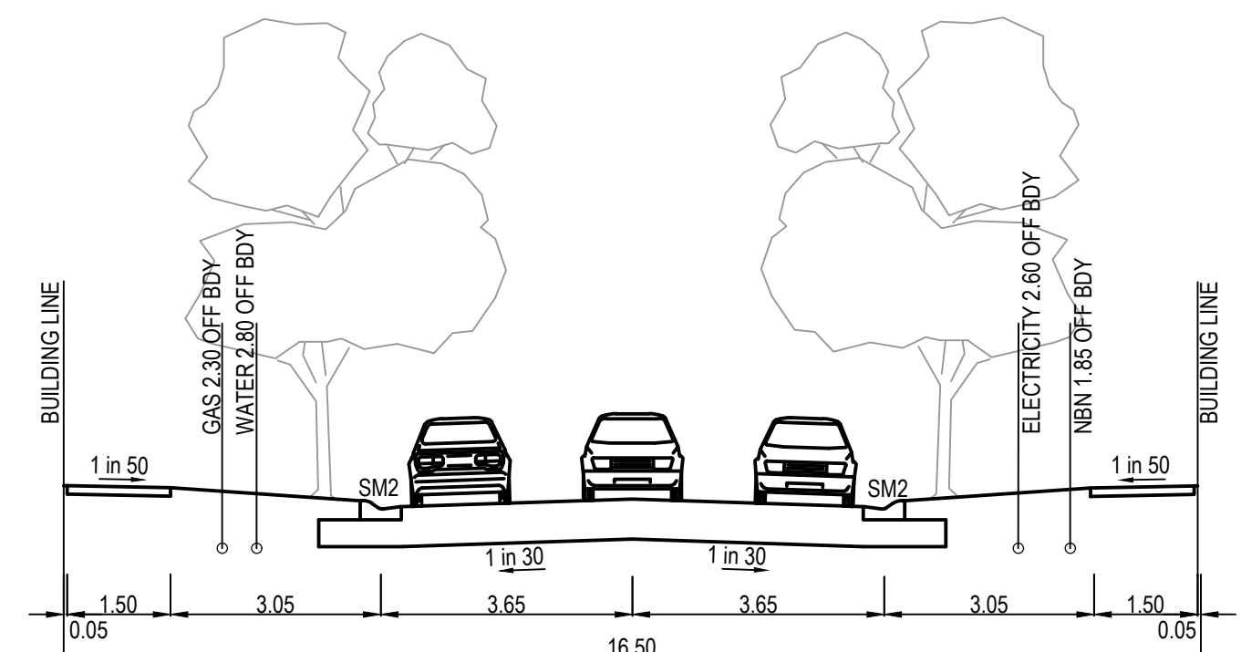
16.5m ROAD RESERVE ACCESS STREET LEVEL 1 TORRANCE DRIVE & ROCKINGHAM CIRCUIT (EAST WEST)
