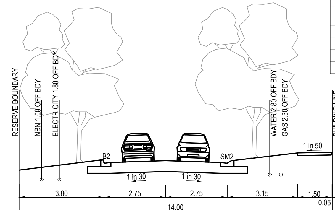
14.0m ROAD RESERVE ACCESS PLACE ROCKINGHAM CIRCUIT (NORTH SOUTH)
