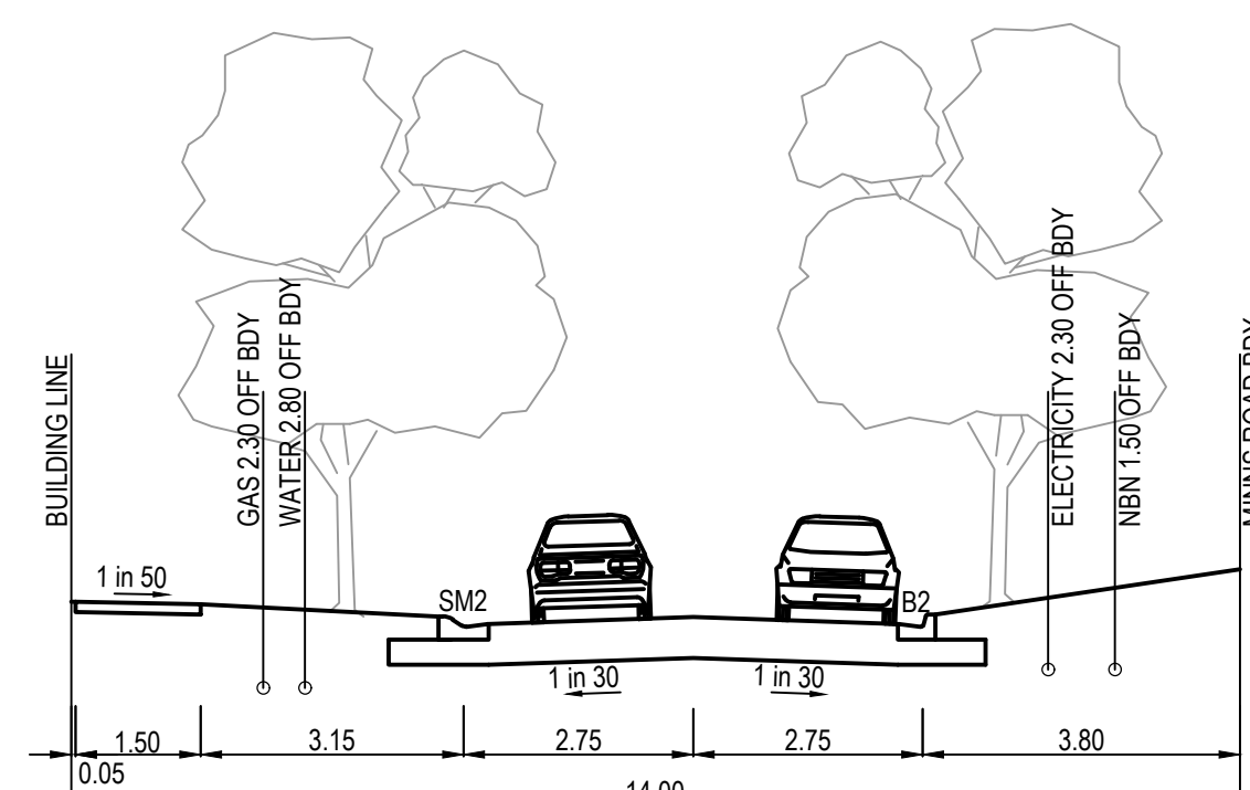
14.0m ROAD RESERVE ACCESS PLACE WYCOMBE ROAD
