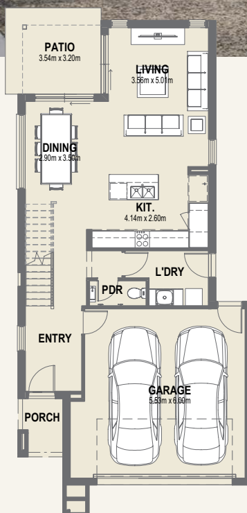
LOWER FLOOR PLAN
