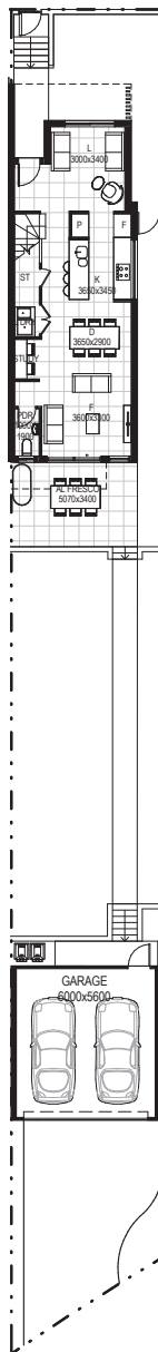
Ground floor
