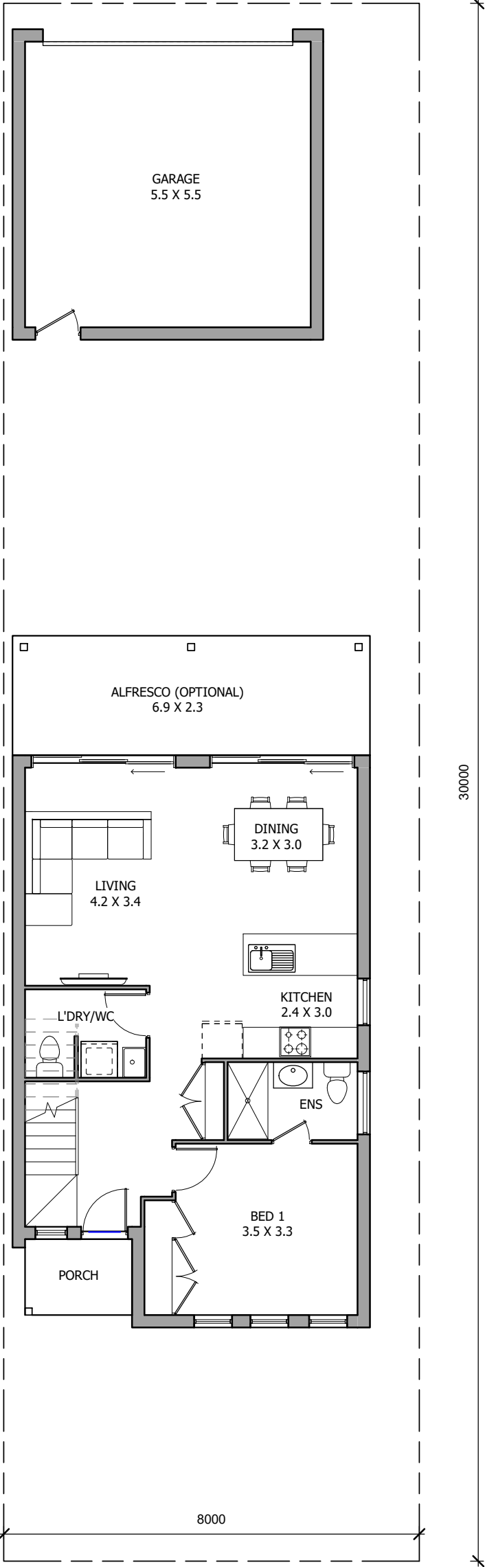
1 GROUND FLOOR SCALE: 1 : 100
