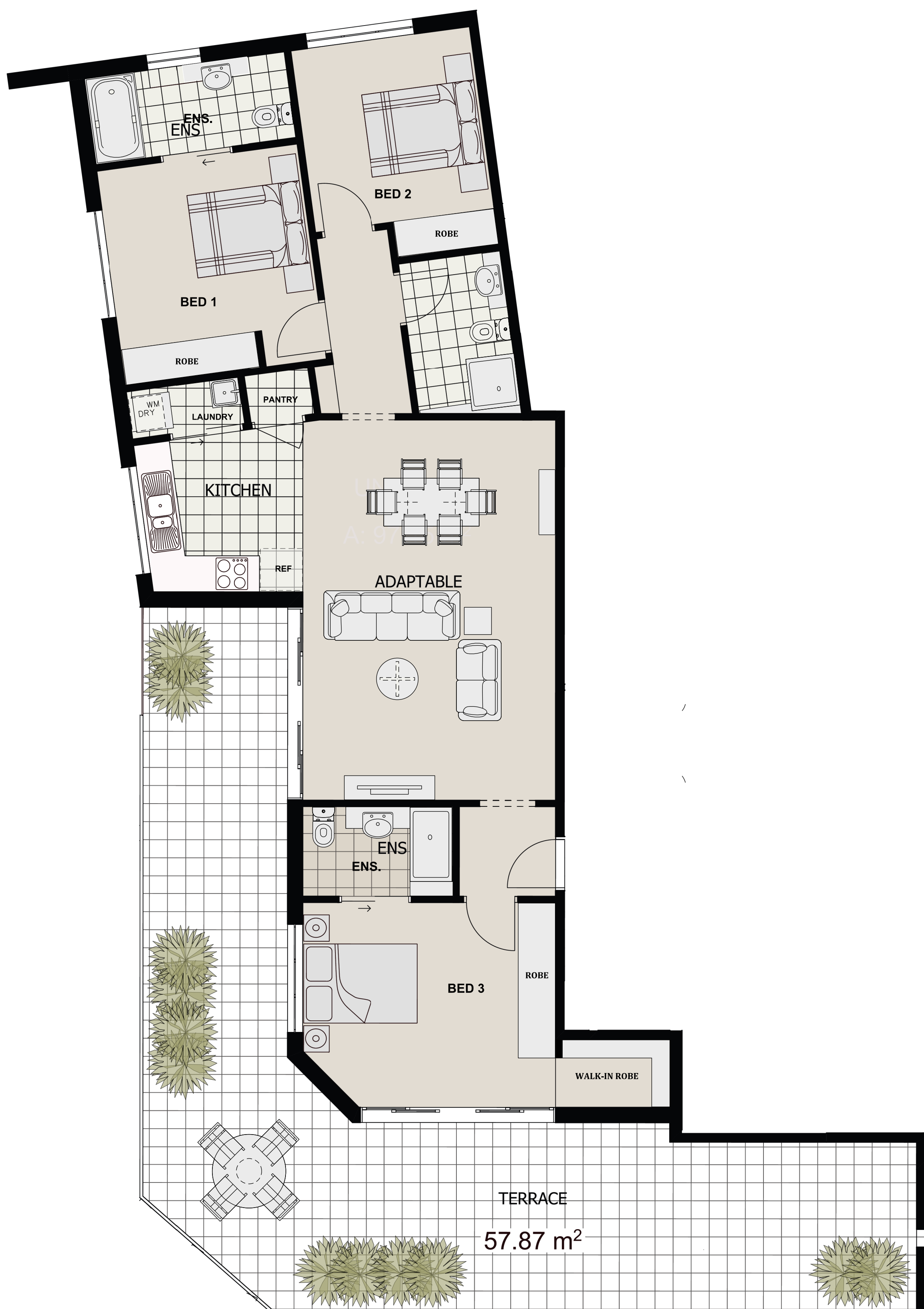
APARTMENT 401, 501 & 601
