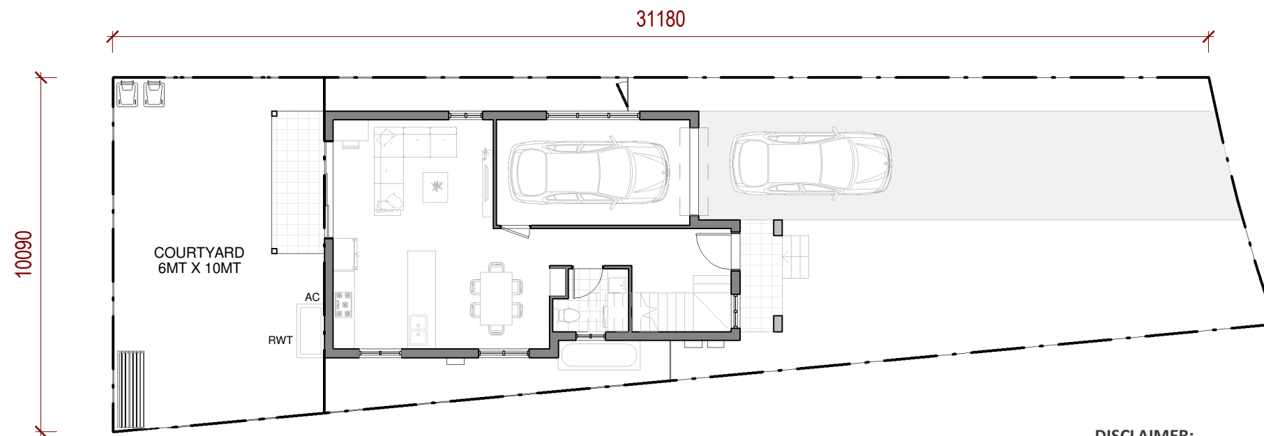
LOT PLAN
